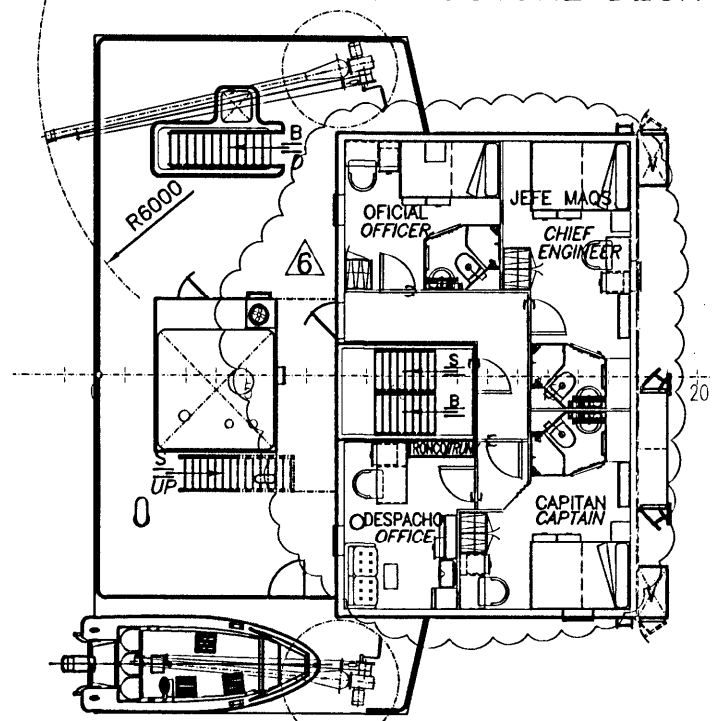
1º CUB. SUPERESTRUCTURA 1st SUPERSTRUCTURE DECK
